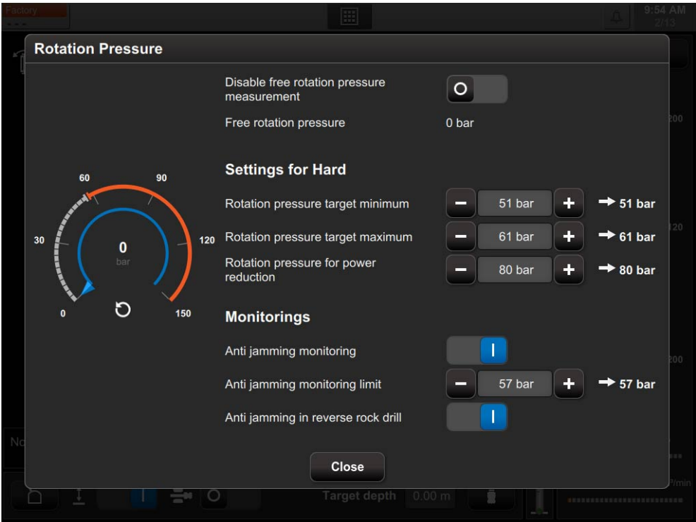
DL rotation pressure, measured
