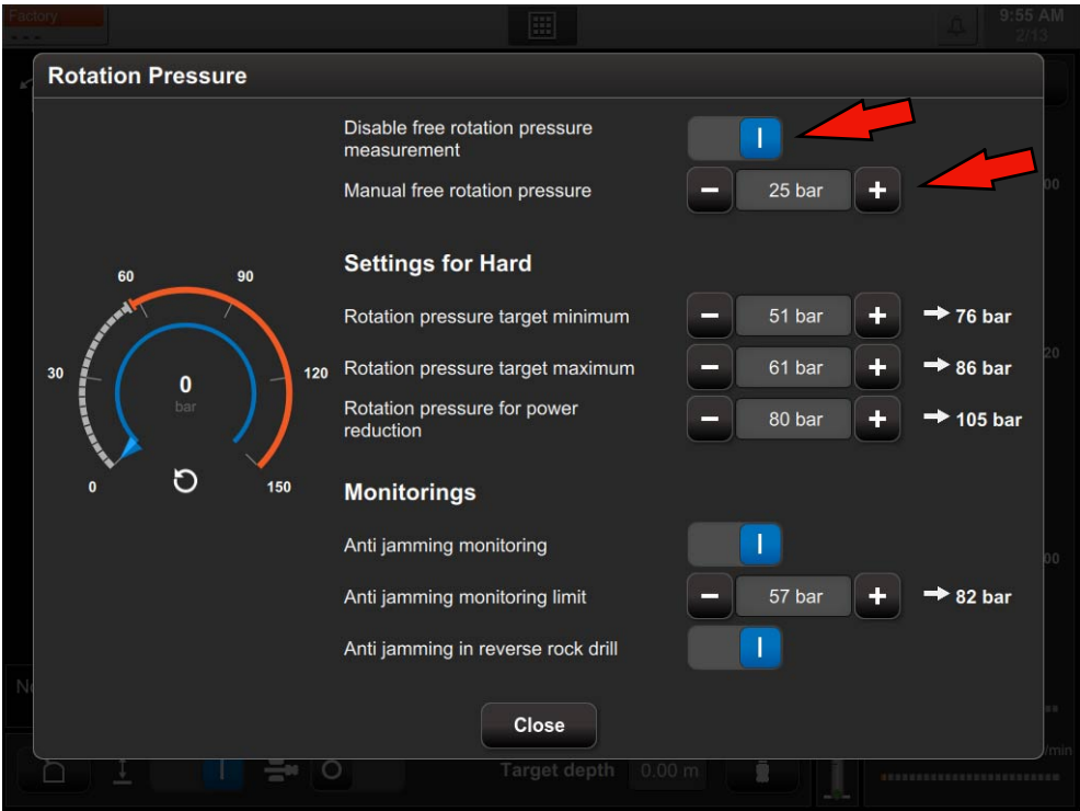
DL rotation pressure, manual
